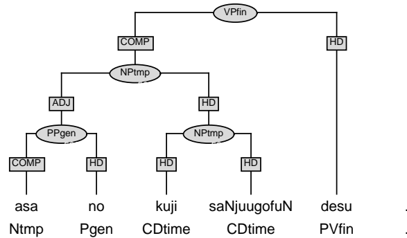
Figure 6.21: Time expression
