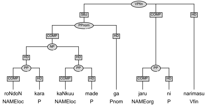
Figure 6.23: From-to expression
