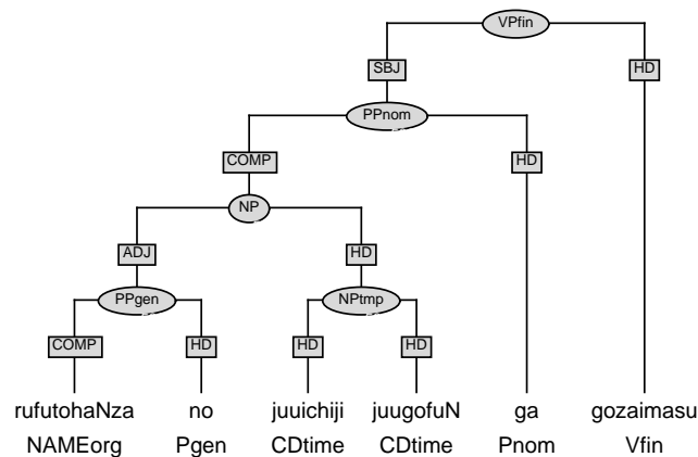
Figure 5.7: Temporal NP?
