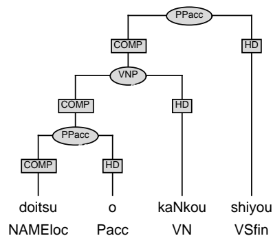
Figure 5.46: VNP suru
