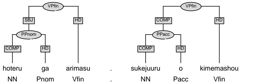
Figure 5.23: Case PP
