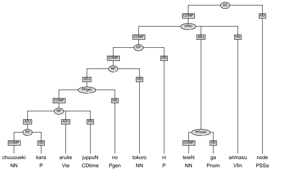
Figure 6.3: Postpositions (COMP-HD)
