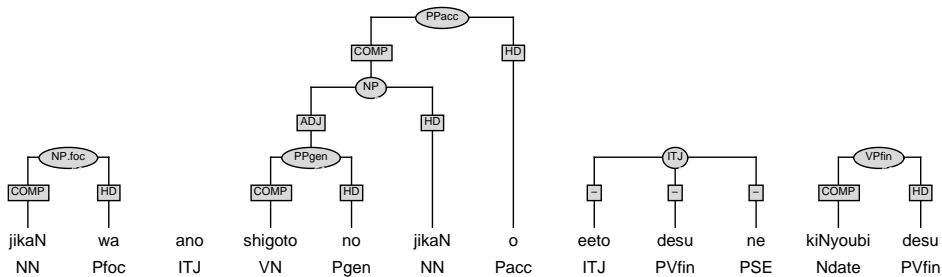
Figure 5.2: Interjections
