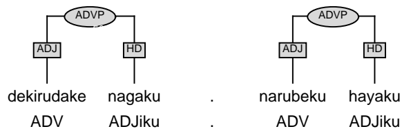
Figure 5.39: ADVP
