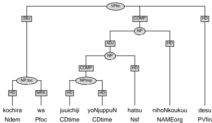
Figure 6.1: Suffixation (COMP-HD)
