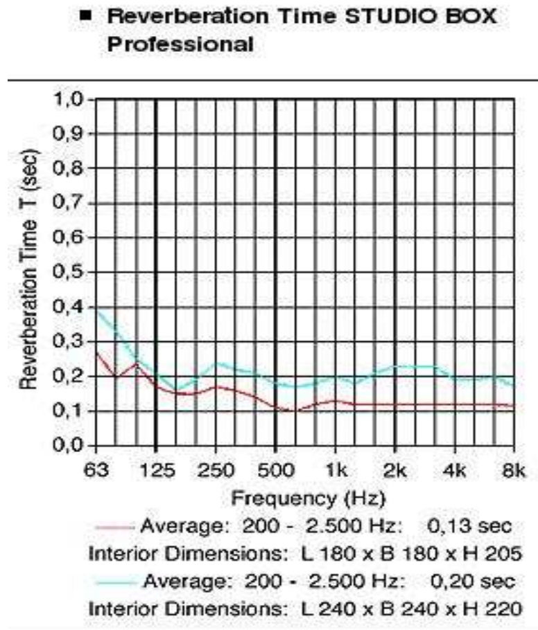
Fig. 1: reverberation time for Studio Box “professional”
